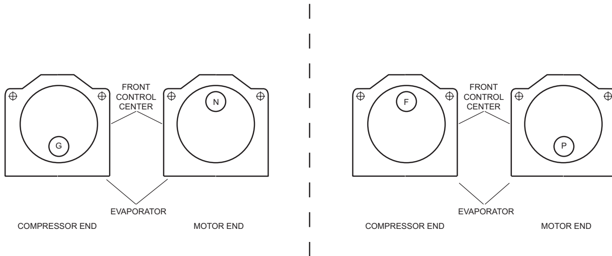
FIG. 6 – 3 PASS
