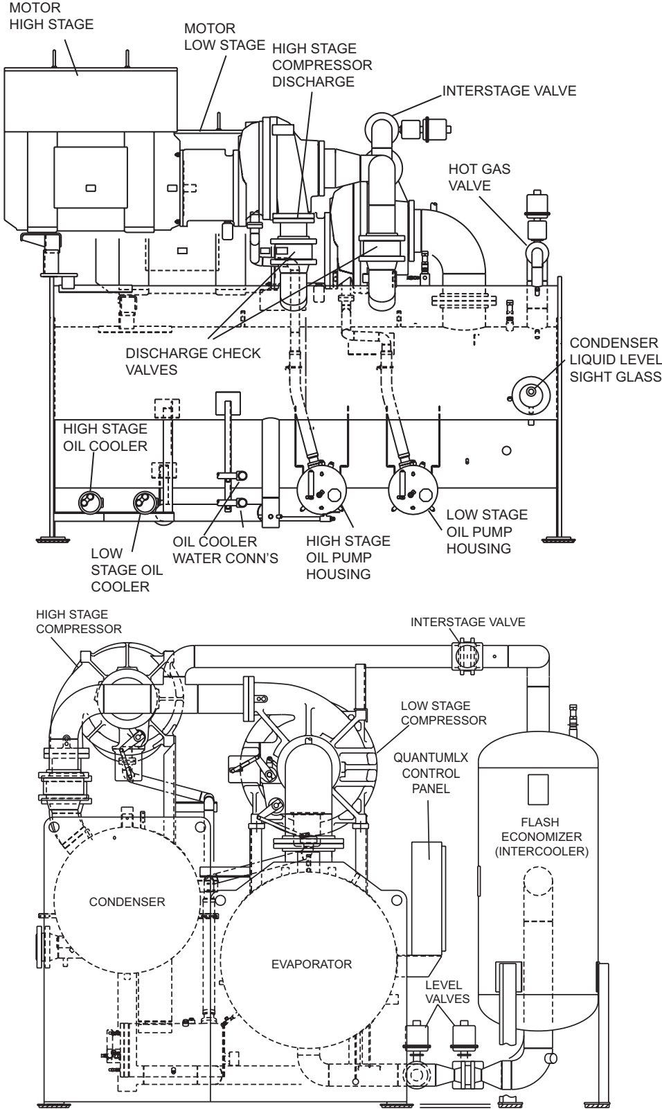
FIG. 2 – UNIT ARRANGEMENT
