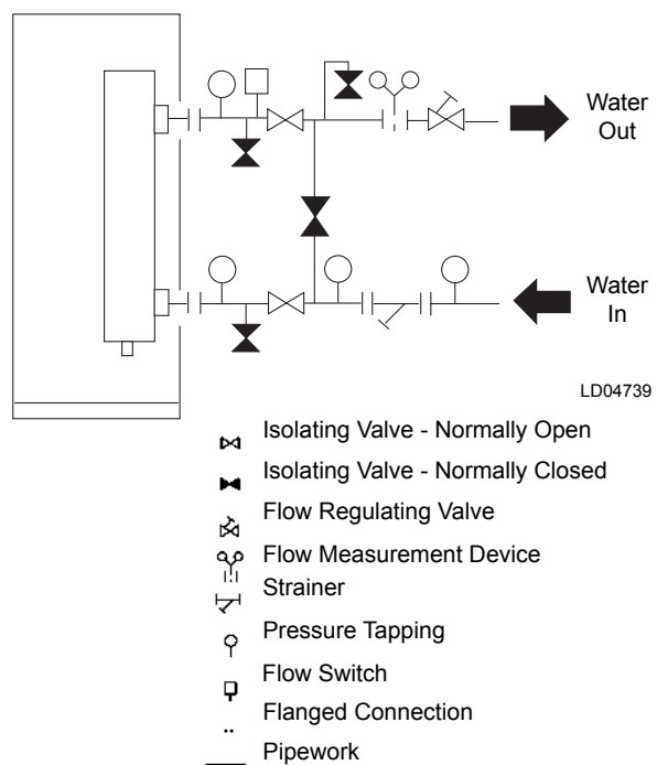
FIG. 6 – PIPEWORK ARRANGEMENT
