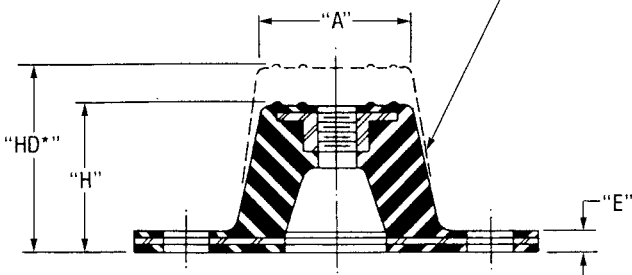
Mounting molded in Neoprene
